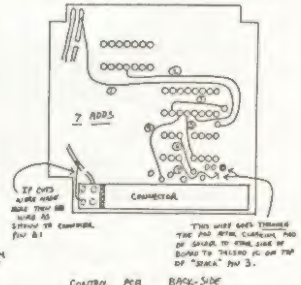
CONTROL PCB BACK-SIDE Illustration D: Adds
